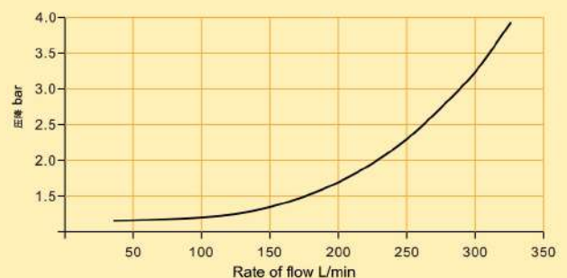
Pressure graph
