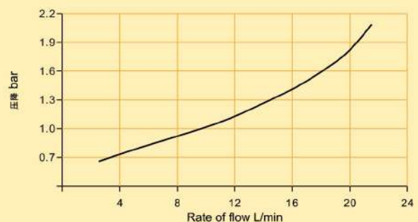
Pressure graph
